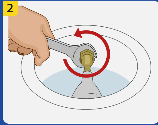
Remove old float valve
