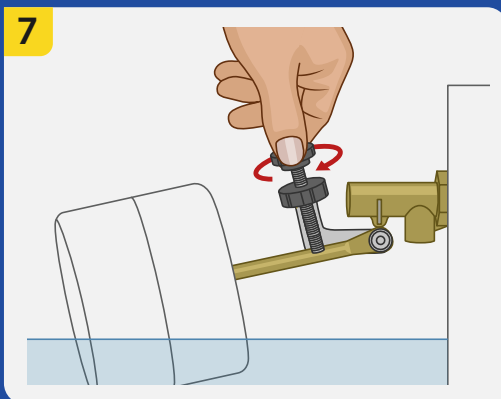
7 Set water level with adjustment knob. Counter clockwise to RAISE the water and clockwise to LOWER the water.
