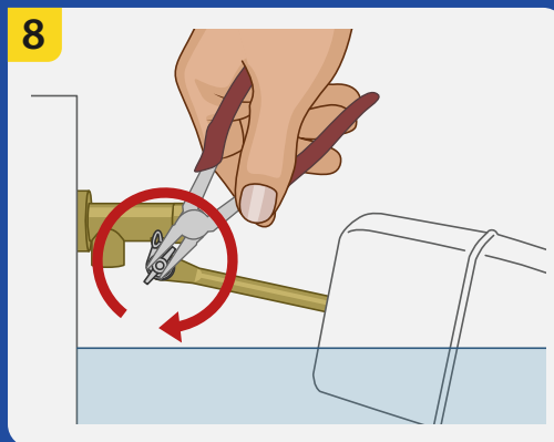
8 Tighten wing nut.
